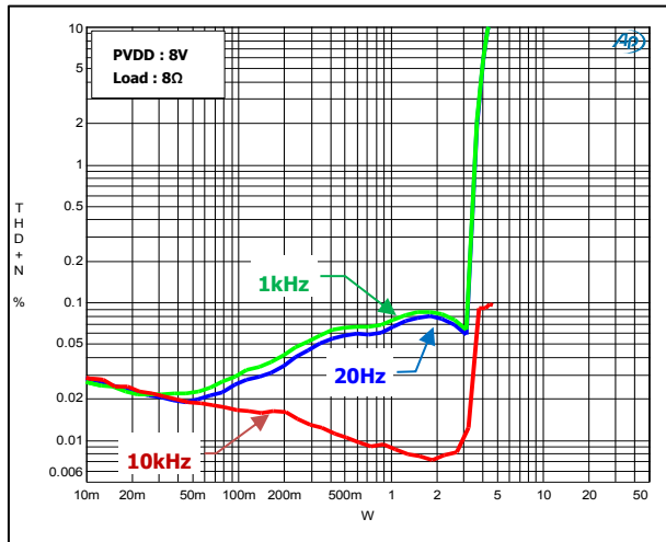
Total Harmonic Distortion + Noise vs. Power, BTL D-BTL Mode Configuration, 8Ω
