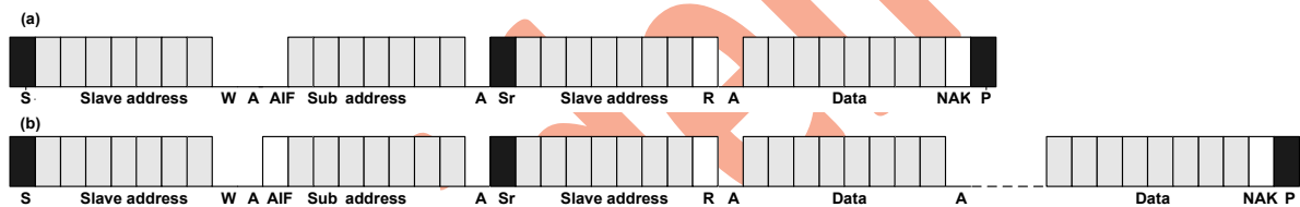
Figure 6. Single Byte Read Mode Sequence
