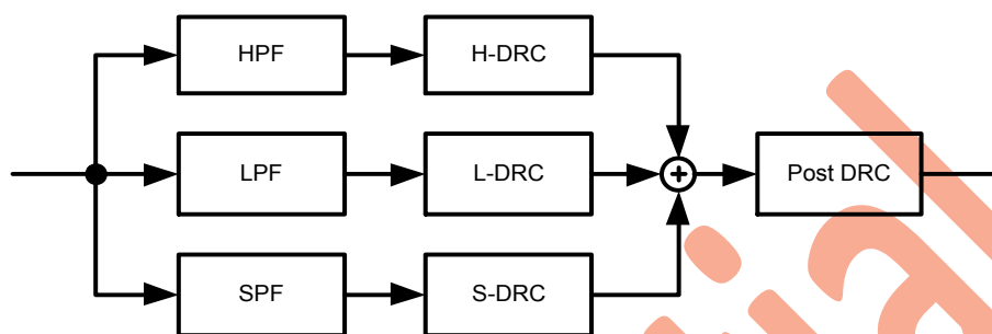
Figure 14. Block Diagram of Dynamic Range Control
