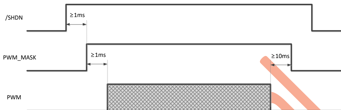
Figure 9. Sound On & Off Sequence
