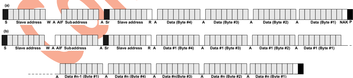
Figure 7. Quad Byte Read Mode Sequence
